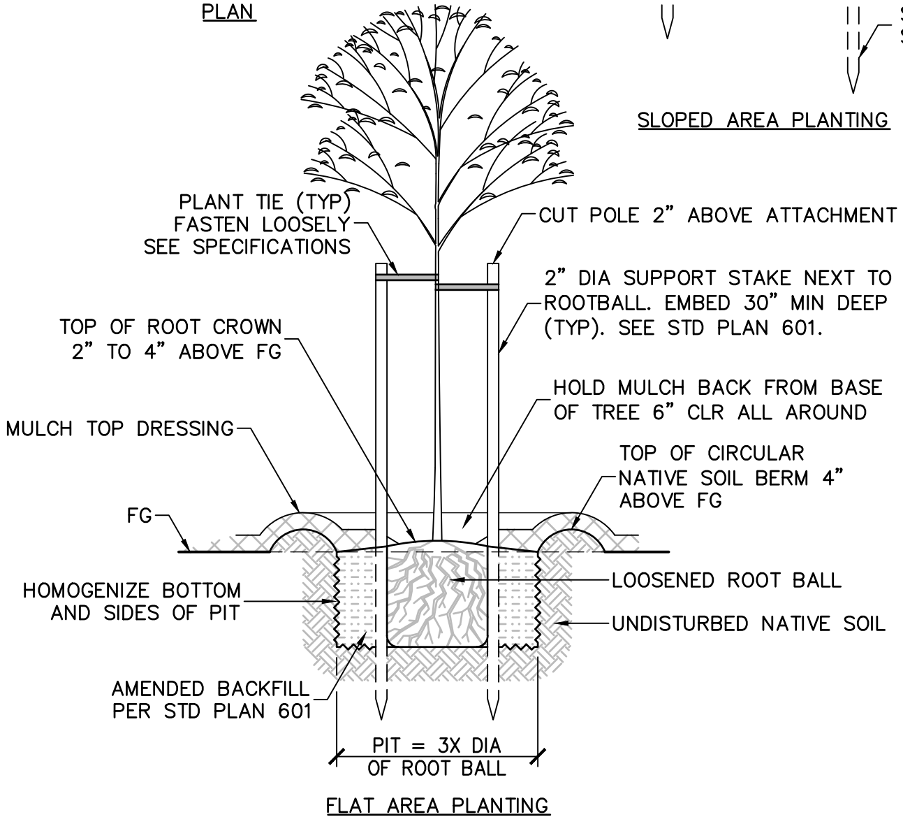
(A) ELEVATION
